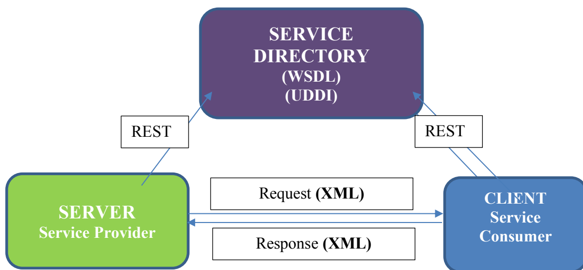
Figure 7.0: Web Services Implementation
