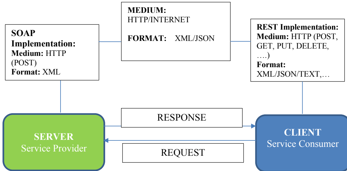
Figure 6.0: SOA concepts
