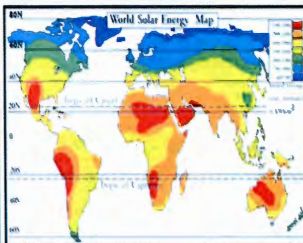
FIGURE 130 : REGIONAL DISTRIBUTION OF SOLAR RADIATION INTENSITY (HTTP://WWW.RISE.ORG.AU/)
